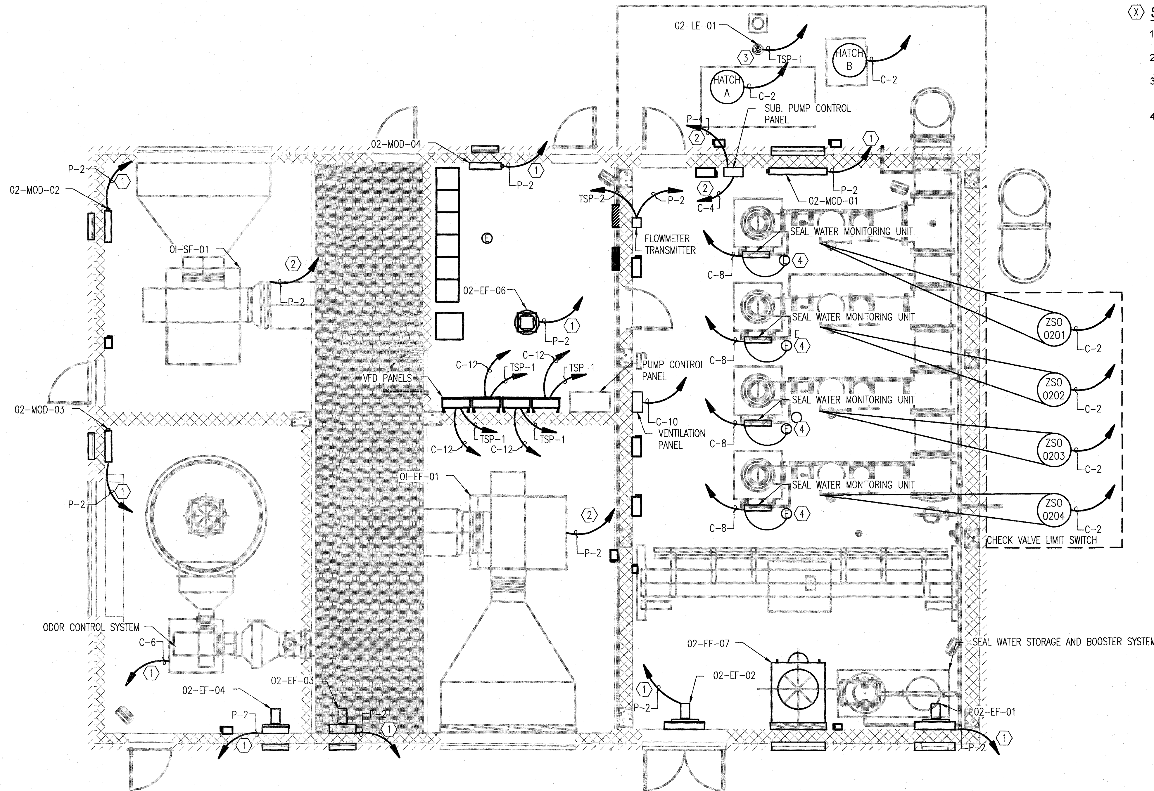
1 PUMP STATION INSTRUMENTATION PLAN GRADE LEVEL 102.09
